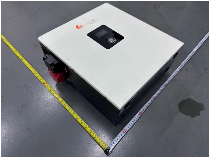
Battery: LPBF24200-A, 25.6V, 200Ah, 5kWh
